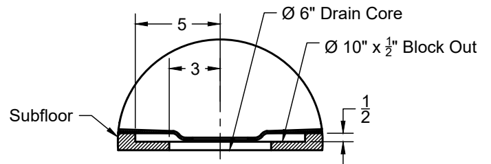
Drain Block-Out
