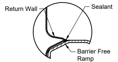
Return Wall Joint
